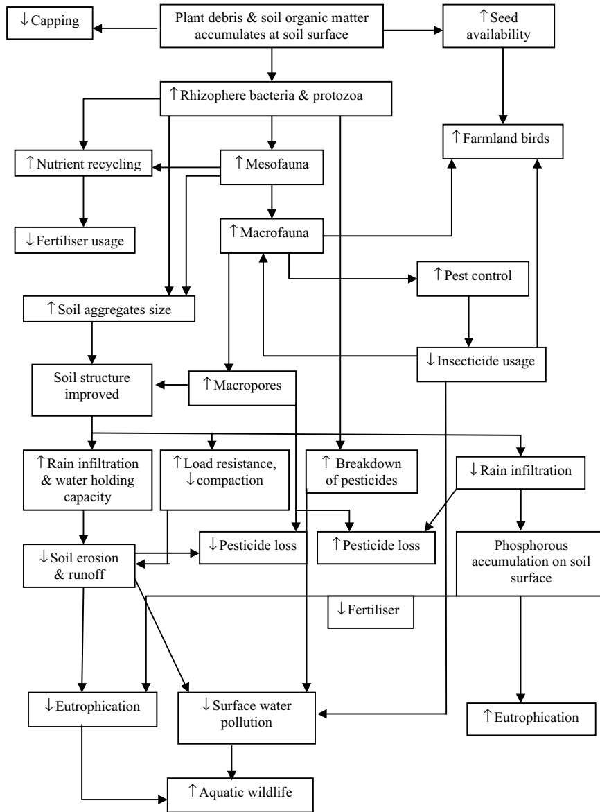
Fig. 2. Interactive processes through which conservation tillage can generate environmental benefits.
